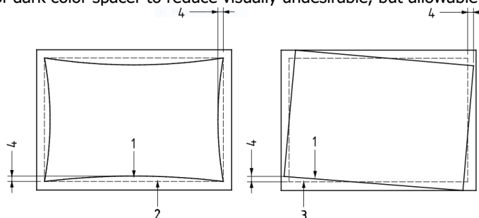
Fig. 6 Examples of spacer deviation
