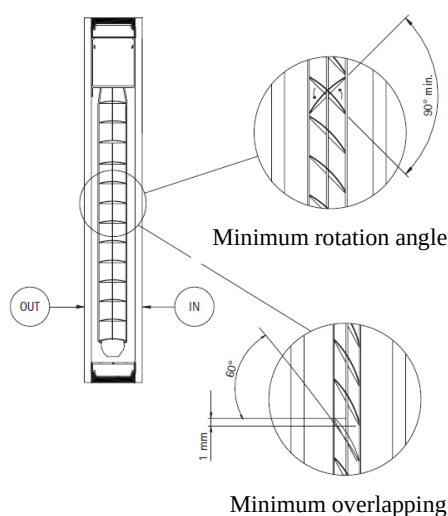
Fig. 18 Overlapping of slats
